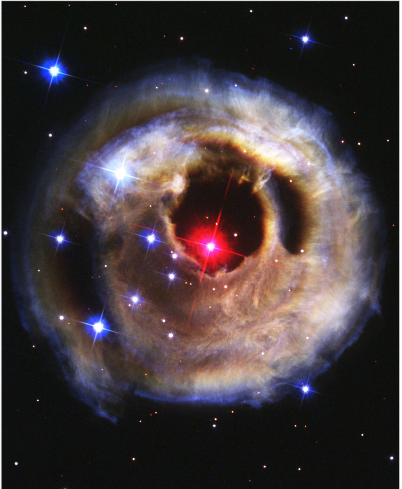
This picture from the NASA/ESA Hubble Space Telescope's Advanced Camera for Surveys dramatically demonstrates the echoing of light through space caused by an unusual stellar outburst in January 2002.
