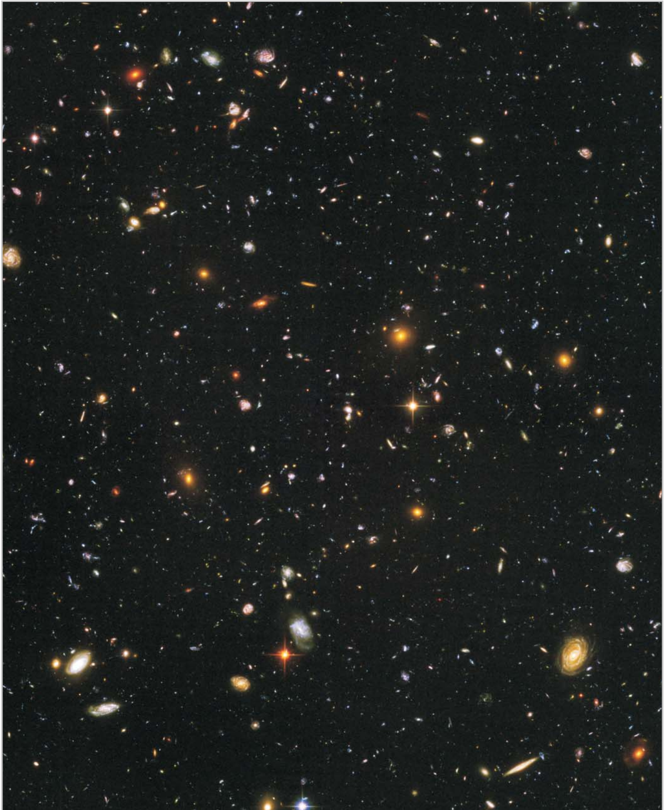
This image is the deepest portrait of the visible Universe ever achieved by humankind. Called the Hubble Ultra Deep Field (HUDF), the million-second-long exposure reveals the first galaxies to emerge from the so-called "dark ages", the time shortly after the big bang when the first stars reheated the cold, dark Universe.
