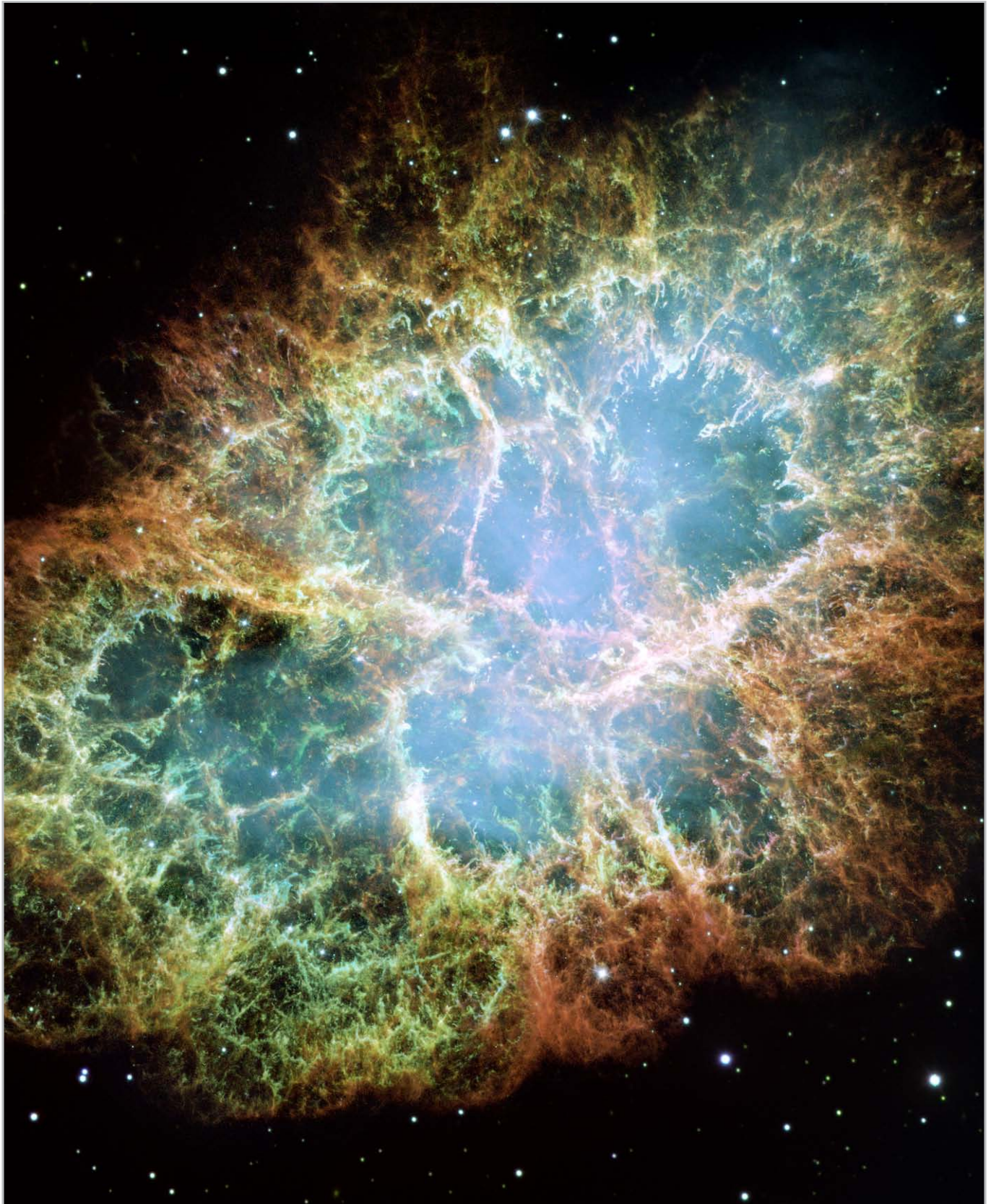
The Crab Nebula is arguably the single most interesting object, as well as one of the most studied, in all of astronomy. The image is the largest ever taken with Hubble's WFPC2 workhorse camera.
