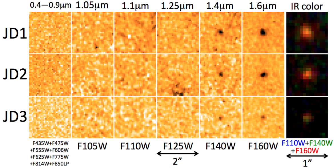
Figure 2. The three images of MACS0647-JD as observed in various filters with HST. The leftmost panels show the summed 11-hour (17-orbit) exposures obtained in 8 filters spanning 0.4–0.9 \mu\text{m} with the Advanced Camera for Surveys. The five middle columns show observations with the Wide Field Camera 3 IR channel in F105W, F110W, F125W, F140W, and F160W, all shown with the same linear scale in electrons per second. The F125W images were obtained at a single roll angle, and a small region near JD2 was affected by persistence due to a moderately bright star in our parallel observations immediately prior (see also Fig. 5). The right panels zoom in by a factor of 2 to show F110W+F140W+F160W color images scaled linearly between 0 and 0.1 \mu\text{Jy} .
