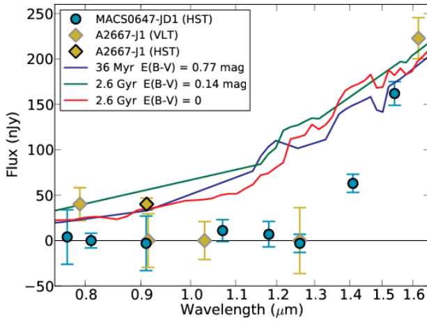
Figure 12. Left: comparison of near infrared photometry of lensed J -dropouts MACS0647-JD1 (this work) and A2667-J1 (Laporte et al. 2011; Hayes et al. 2012). Also overlotted are three SED fits from Figure 2 of Hayes et al. (2012) to the photometry of A2667-J1 at its spectroscopic redshift z = 2.082 . The Hayes et al. (2012) photometry plotted here is all from VLT (FORIS2 and HAWK-I) except for the 6.0\text{-}\sigma detection in HST/ACS F850LP, the upper diamond with a darker border at 0.91\mu\text{m} . Right: photometric redshift probability distribution for A2667-J1 based on our reanalysis of the photometry provided in Hayes et al. (2012) with and without a Bayesian prior. The top panel uses all the available photometry. The middle panel omits the 6.0\text{-}\sigma detection in ACS/F850LP. The bottom panel omits both ACS and Spitzer IRAC ch3 and ch4. The spectroscopic redshift z = 2.082 is indicated by the red vertical lines.
