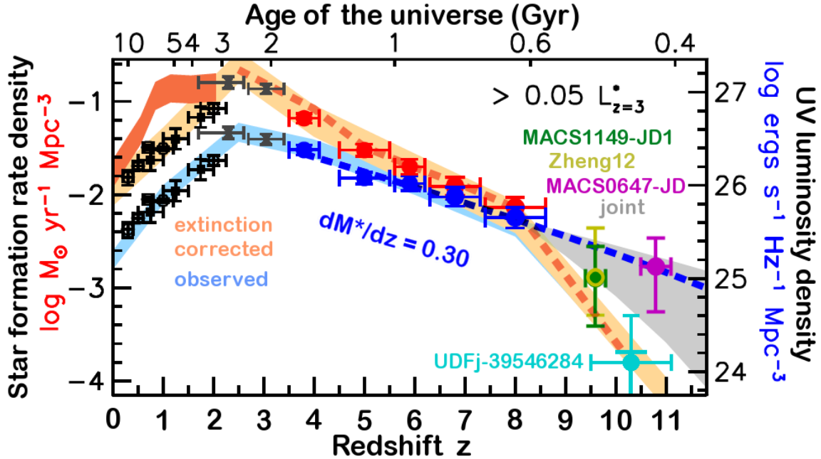
Figure 18. CLASH constraints on the cosmic star formation rate density at z \sim 9.6 and 11.0 compared to previous estimates from 0 \lesssim z \lesssim 10 as compiled and corrected for dust extinction by Bouwens et al. (2012b). We adopt the z \sim 8 LF from Bradley et al. (2012b) and assume M^* evolves with linearly redshift. MACS0647-JD constrains dM^*/dz = 0.30^{+0.25}_{-0.18} , while MACS1149-JD1 (Zheng et al. 2012) constrains dM^*/dz = 0.62^{+0.43}_{-0.33} , yielding a joint constraint of dM^*/dz = 0.40^{+0.23}_{-0.17} . We integrate these LFs down to 0.05L^*(z=3) , or M_{UV,1400} \approx -17.7 AB mag, to obtain rest-frame UV luminosity densities (magenta and green points with the gray shaded region giving the joint constraint). The yellow point is an alternative estimate of the z \sim 9.6 SFRD from Zheng et al. (2012) rescaled by 12/17 to account for the larger search volume behind 17 clusters. An extrapolation from z \sim 8 assuming dM^*/dz = 0.30 is shown as the dashed blue line. Points along the bottom blue curve are observed while the upper orange curve is corrected for extinction by Bouwens et al. (2012b). We assume a star formation rate of one solar mass per year produces a UV ( 0.14\mu\text{m} ) luminosity of 8 \times 10^{27} ergs \text{s}^{-1} \text{Hz}^{-1} (right axis), as from a Salpeter (1955) IMF truncated between 0.1 and 125 M_{\odot} . A Chabrier (2003) IMF would yield lower SFRD by a factor of \sim 1.8 . Previous data are from Schiminovich et al. (2005); Oesch et al. (2010b); Reddy & Steidel (2009); Bouwens et al. (2007, 2011a); Oesch et al. (2012a) as described in Bouwens et al. (2012b, see their Fig. 19).
