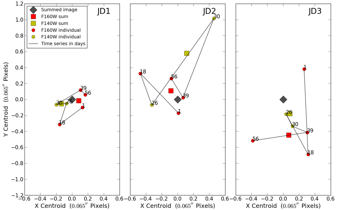
Figure 6. Relative centroid measurements for the detections in F160W (red) and F140W (yellow) in individual epochs (circles) and summed observations (squares). Centroids measured in the summed NIR images are also plotted as gray diamonds. The offsets are generally less than one of our drizzled pixels ( 0.065'' ), roughly half the native WFC3/IR pixel size ( \sim 0.13'' ).
