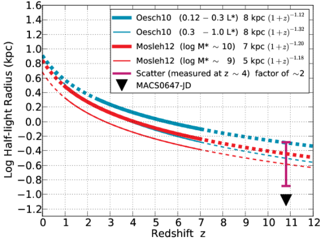
Figure 16. Upper limit on MACS0647-JD half-light radius (deconvolved and delensed) compared to observed mean galaxy sizes from Oesch et al. (2010a) and Mosleh et al. (2012) extrapolated to z \sim 11 . The intrinsic scatter in galaxy sizes is a factor of \sim 2 as measured for well-studied samples at z \sim 4 (Ferguson et al. 2004).
